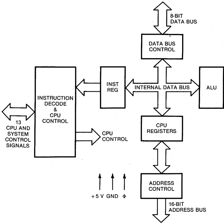
Fig. 4-2. Block diagram of Z80. (Courtesy MOSTEK Corp.)
